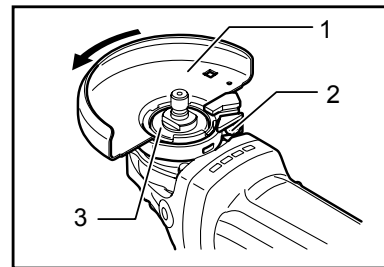
1. Wheel guard 2. Screw 3. Bearing box
